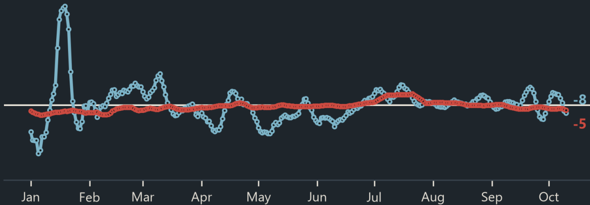
PM10 residual, 2026
