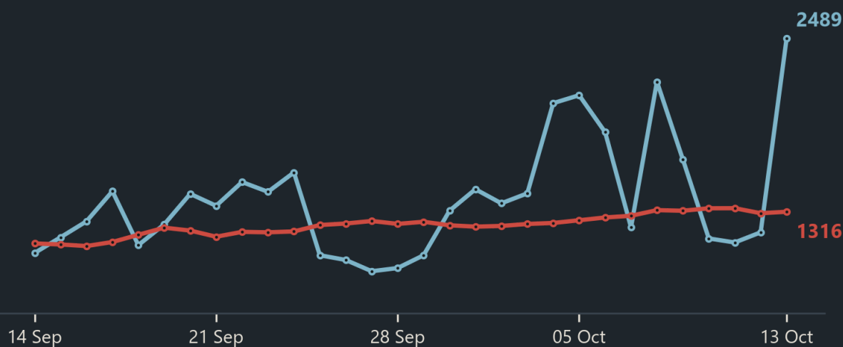
CO, daily level, not a residual ( \mu\text{g}/\text{m}^3 )
