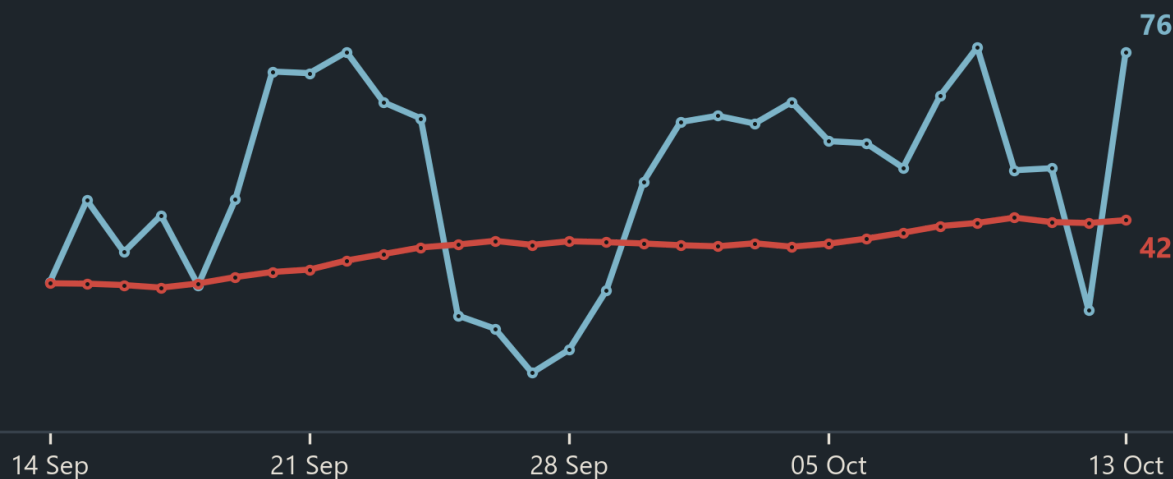
PM2.5, daily level, not a residual ( \mu\text{g}/\text{m}^3 )
