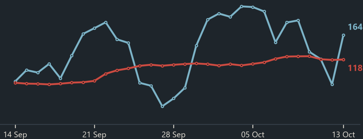
PM10, daily level, not a residual ( \mu\text{g}/\text{m}^3 )
