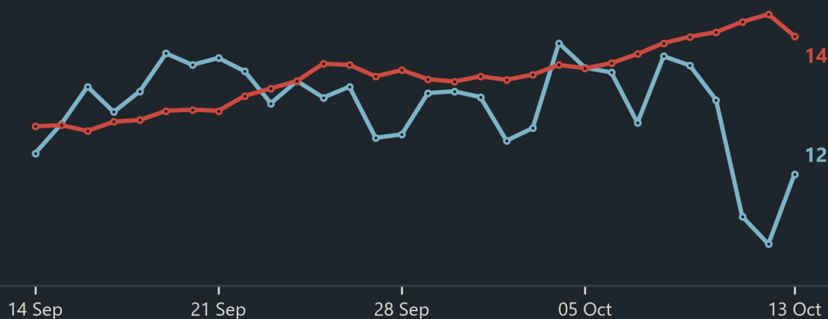
CO, daily level, not a residual ( \mu\text{g}/\text{m}^3 )
