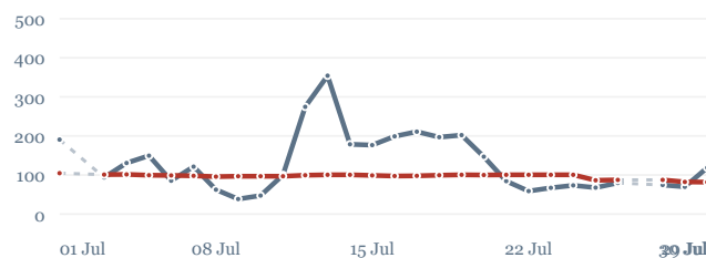
NO x · daily level, not a residual
