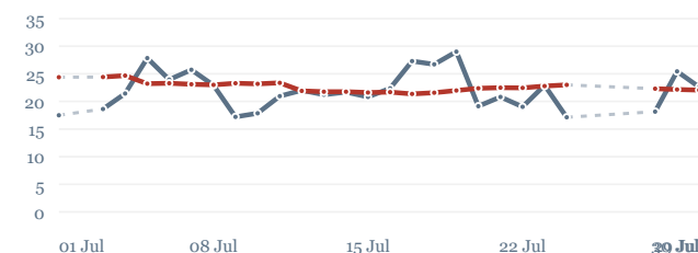
CO · daily level, not a residual
