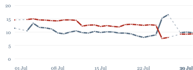
Ozone · daily level, not a residual
