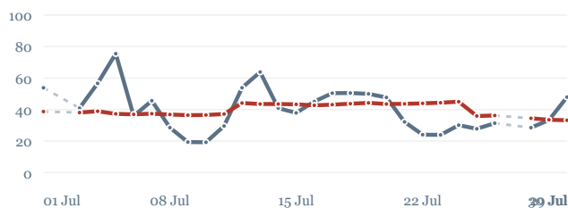
NO 2 · daily level, not a residual
