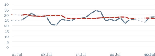
SO 2 · daily level, not a residual
