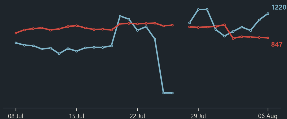
CO, daily level, not a residual (µg/m 3 )
